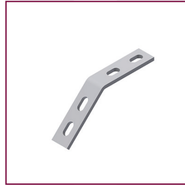
Bevel for T- shaped stanchion made of flat steel 30x6 mm, leg length 100x100 mm, inclination 45°
