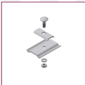
Side connector for a straight connection of C-grid cable trays, dimension 60x41 mm, completely assembled with truss-head screw, washer and nut
